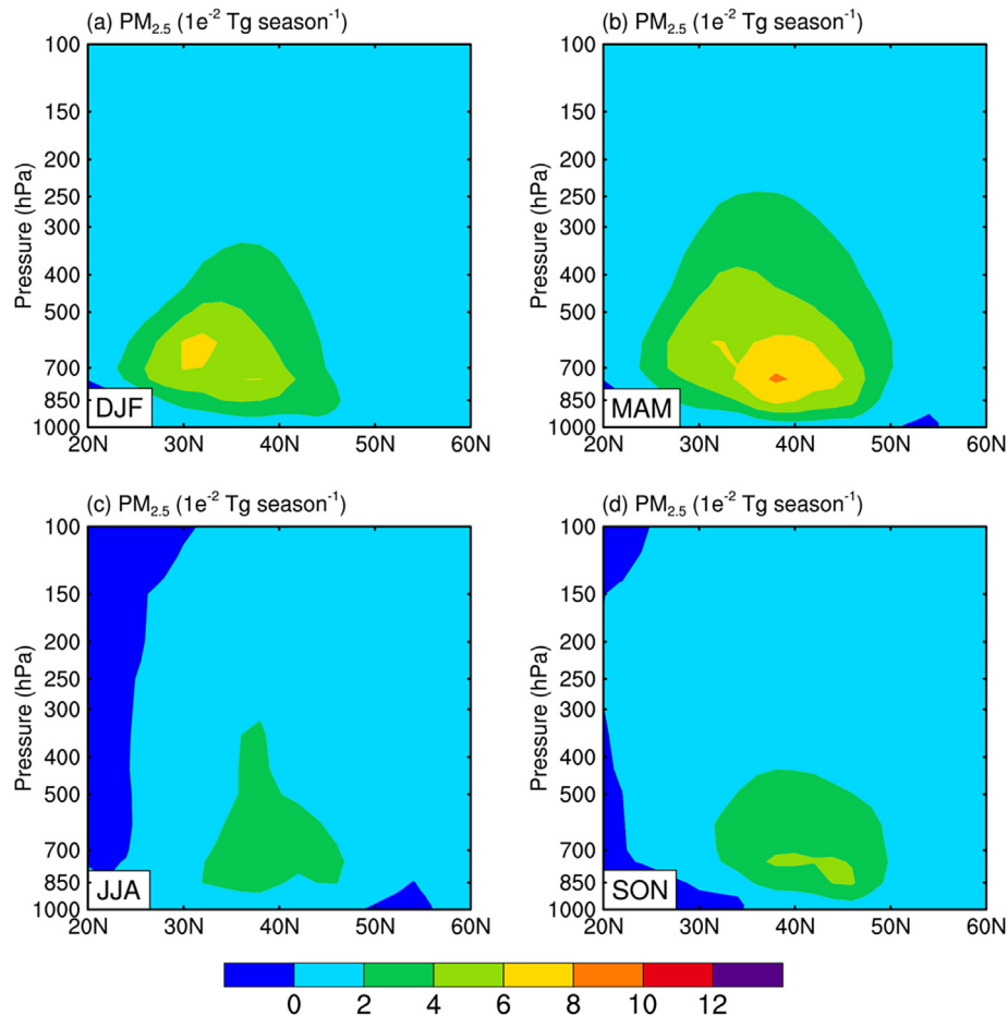
Fig. 3. Simulated seasonal outflow fluxes of PM_{2.5} across the selected plane along 135^\circ E from 20^\circ to 60^\circ N that are averaged over years 1986–2006 of simulation VALL. Positive values represent eastward fluxes and negative values represent westward fluxes.
