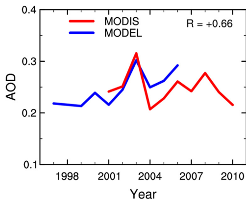
Fig. 4. Comparison simulated aerosol optical depth (AOD) with MODIS AOD. Both the simulated and observed AOD values are the averages over the selected region ( 30^\circ – 50^\circ N , 130^\circ – 150^\circ E ) in the western Pacific Ocean. The MODIS datasets are available since year 2001, and modeled AOD values from simulation VALLB (with variations in meteorological parameters as well as anthropogenic and biomass burning emissions) are available for 1997–2006. Correlation coefficient R between simulations and observations is calculated over the time period of 2001–2006.
