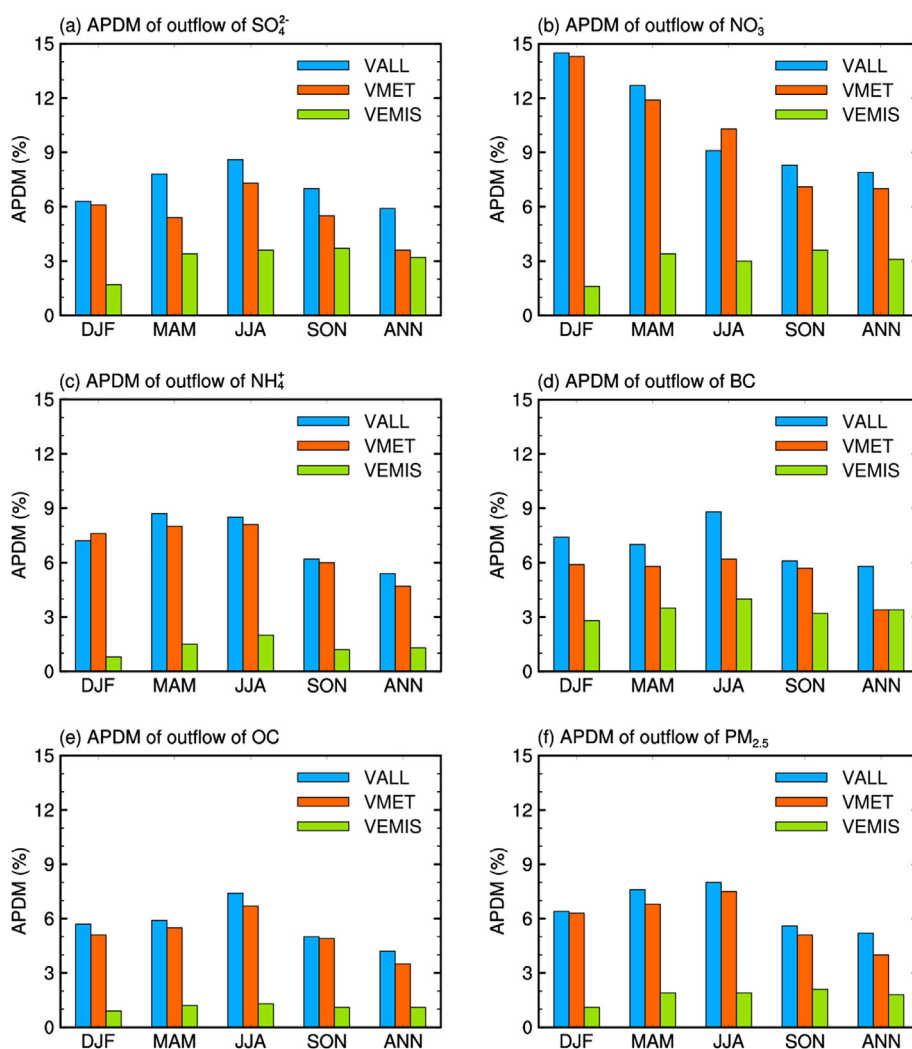
Fig. 7. The APDM values of the detrended seasonal and annual outflow fluxes of (a) \text{SO}_4^{2-} , (b) \text{NO}_3^- , (c) \text{NH}_4^+ , (d) BC, (e) OC, and (f) \text{PM}_{2.5} from simulations VALL, VMET, and VEMIS for 1986–2006.
