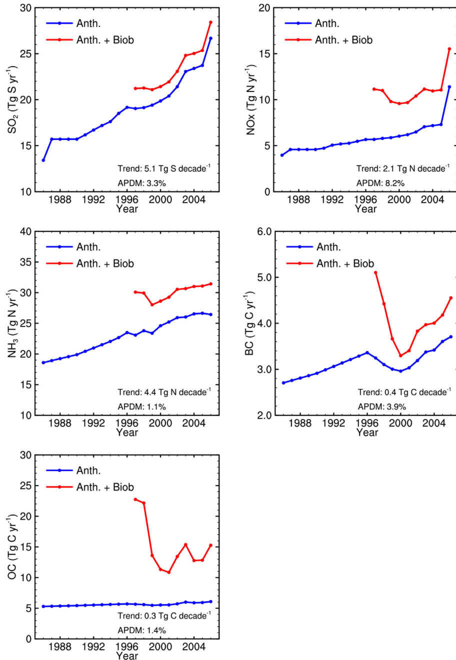
Fig. 1. Yearly variations in anthropogenic and biomass burning emissions of (a) \text{SO}_2 , (b) \text{NO}_x , (c) \text{NH}_3 , (d) BC, and (e) OC in Asia ( 60^\circ\text{E} – 150^\circ\text{E} , 10^\circ\text{S} – 56^\circ\text{N} ) over years 1986–2006. Blue lines are anthropogenic emissions and red lines represent total emissions (anthropogenic plus biomass burning emissions). The linear trend and absolute departure from the mean (APDM) of anthropogenic emissions are shown at the bottom right corner of each panel. Note that biomass burning emissions are not available before year 1997. (For interpretation of the references to color in this figure legend, the reader is referred to the web version of this article.)
