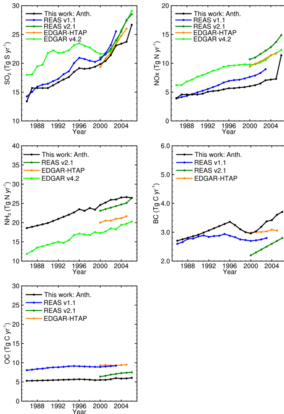
Fig. 8. Comparisons of the yearly variations in regional total anthropogenic emissions used in this work with those from other emissions inventories for (a) \text{SO}_2 , (b) \text{NO}_x , (c) \text{NH}_3 , (d) BC, and (e) OC. See Table 3 for the detailed information of these emissions inventories.
