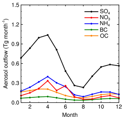
Fig. 2. Monthly outflow fluxes of different aerosol species from simulation VALL that are averaged over years 1986–2006.
