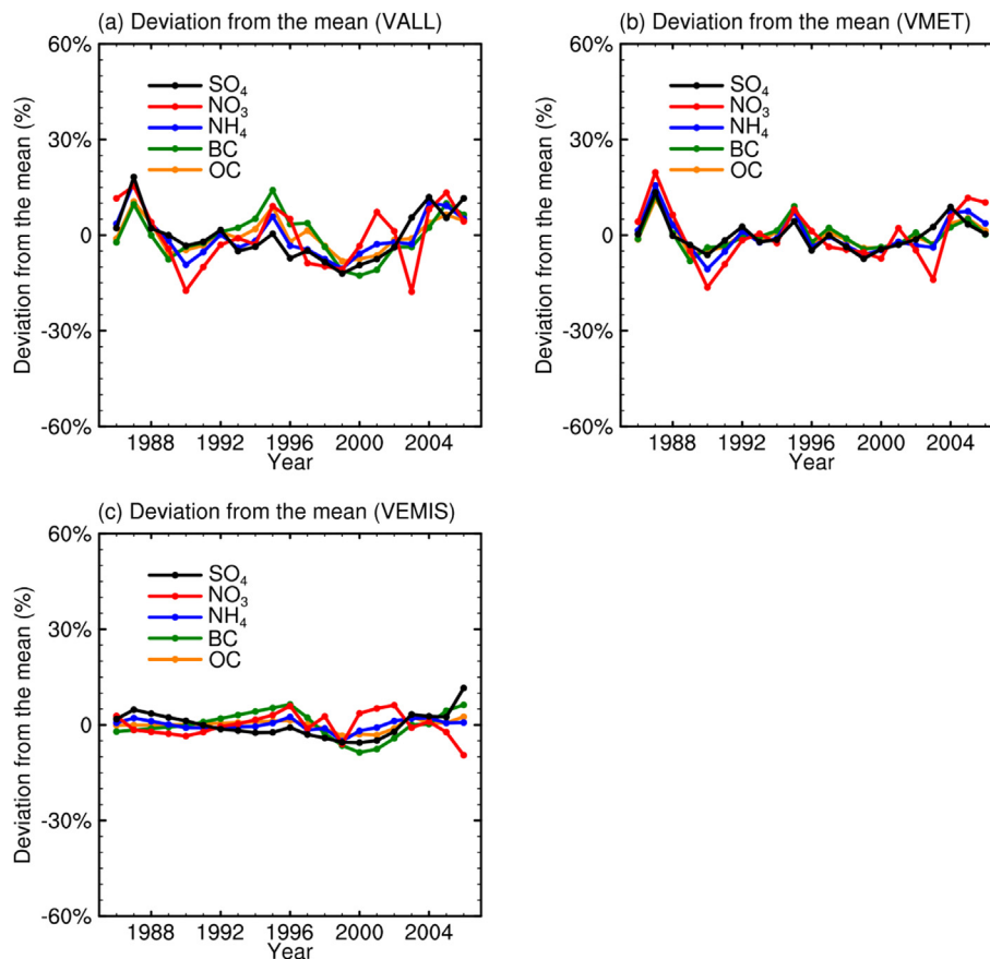
Fig. 6. Deviation from the mean of the detrended outflow fluxes of different aerosol species from simulations (a) VALL, (b) VMET, and (c) VEMIS for 1986–2006.
