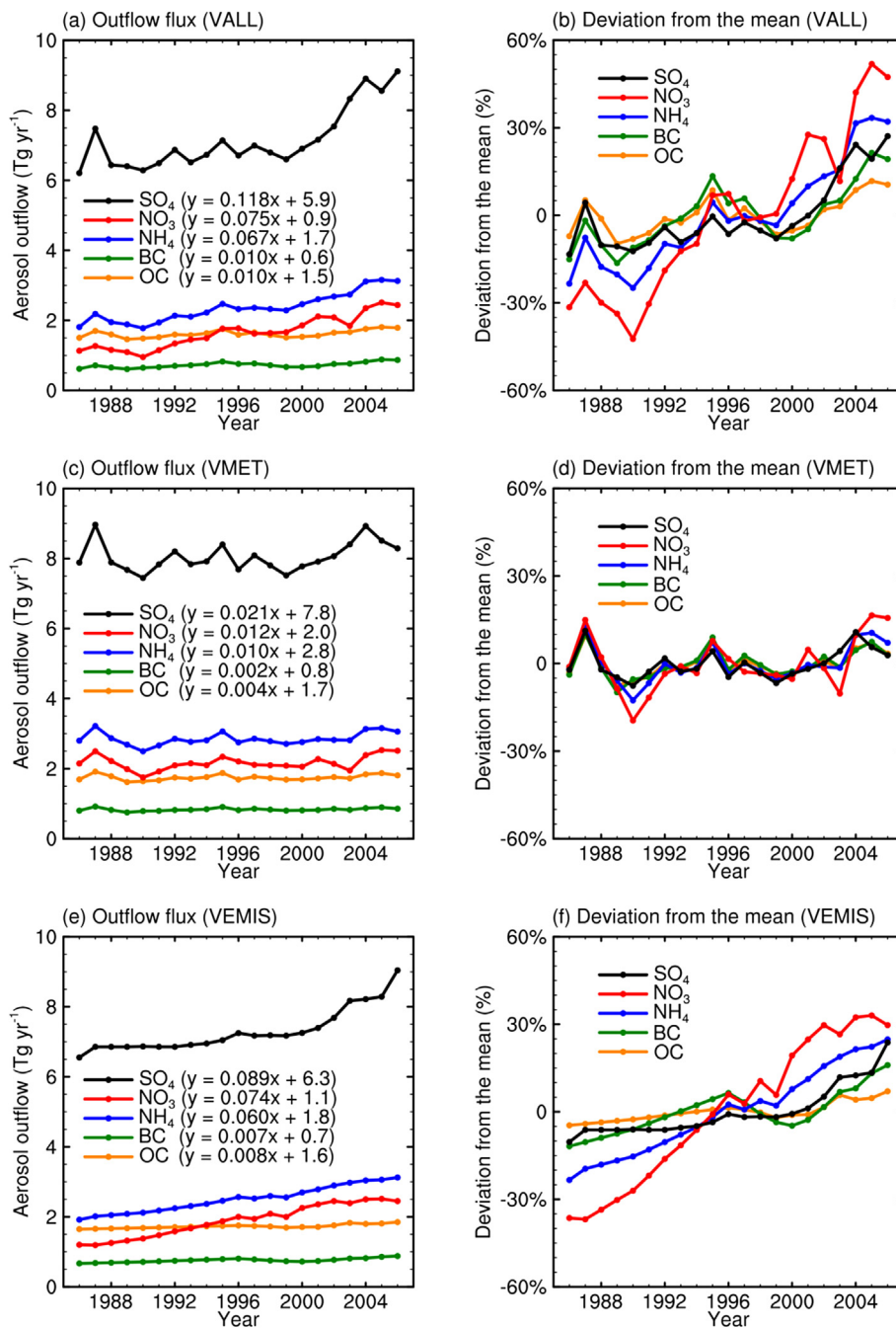
Fig. 5. Annual aerosol outflow fluxes from East Asia for years 1986–2006 simulated in simulations (a) VALL, (c) VMET, and (e) VEMIS with the associated deviation from the mean in (b), (d) and (f), respectively. The decadal trends in outflow fluxes are calculated using the least square fit approach and are presented in parenthesis in (a), (c), and (e). See text for the definition of deviation from the mean.
