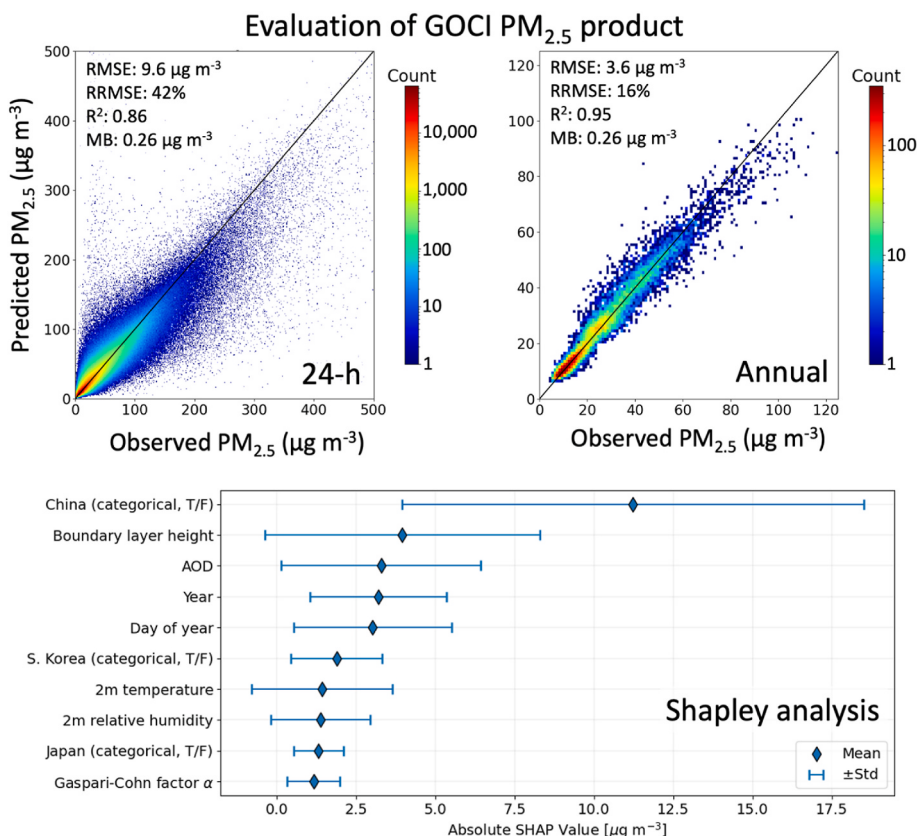
Fig. 4. Evaluation of the GOCI \text{PM}_{2.5} RF predictions. The top panels evaluate the GOCI \text{PM}_{2.5} RF predictions in the 2011–2022 training period at grid cells withheld entirely from training in a ten-fold crossvalidation procedure, aggregated at (a) 24-h and (b) annual resolution. The panels show two-dimensional histograms where pixel color corresponds to the count of observation/prediction correspondences within the corresponding bin, with statistics inset and the identity line shown in black. The bottom panel shows the top ten predictors of GOCI \text{PM}_{2.5} ranked by importance by the SHAP analysis. Predictor variable contributions are shown by mean absolute SHAP values and standard deviations. (For interpretation of the references to color in this figure legend, the reader is referred to the Web version of this article.)
