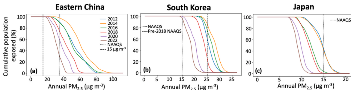
Fig. 10. Trends in cumulative population exposure in countries within the study domain. The y axis shows the cumulative populations exposed to at least the annual \text{PM}_{2.5} level given on the x axis, with year indicated by color. Panel (a) shows Eastern China, (b) South Korea, and (c) Japan. Note different scales for the different panels. National ambient air quality standards (NAAQS) are shown in the vertical black dotted line. (For interpretation of the references to color in this figure legend, the reader is referred to the Web version of this article.)
