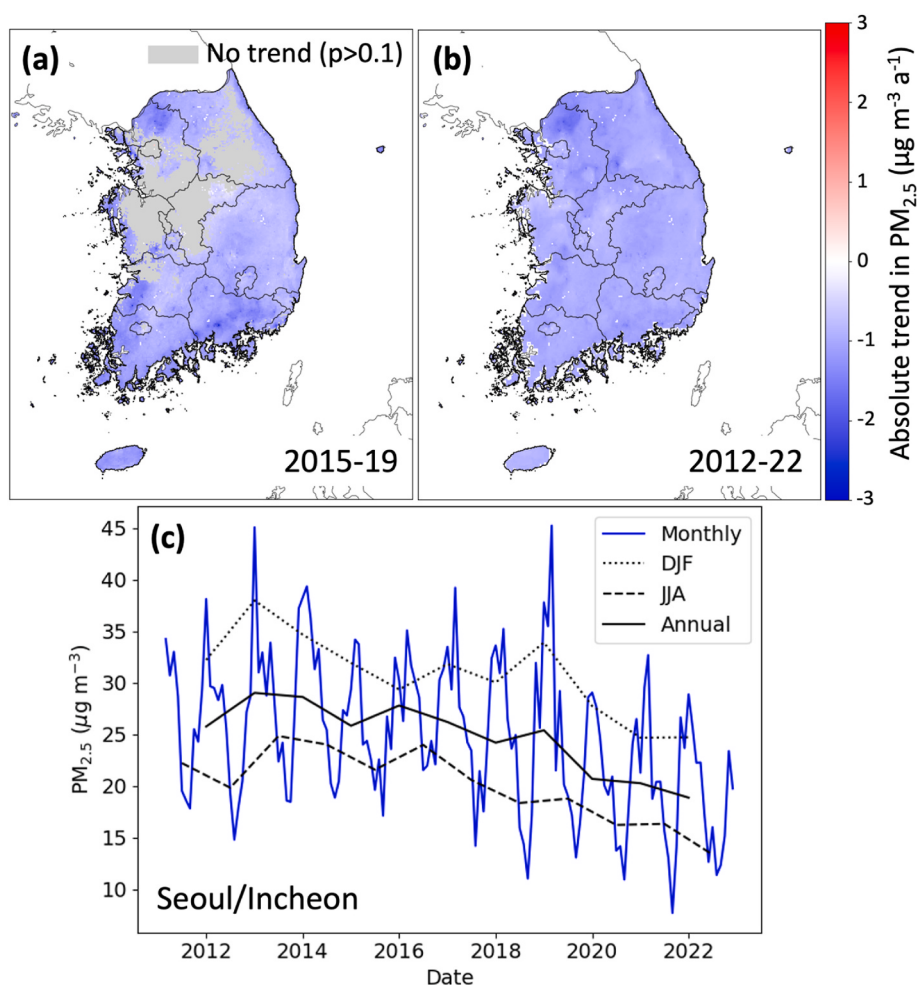
Fig. 9. Trends in PM_{2.5} concentrations in South Korea. Panels in the top row show annual trends for (a) 2015–2019 and (b) 2012–2022. The trends are obtained by ordinary linear regression of the annual mean GOCI PM_{2.5} in each 2 \times 2 \text{ km}^2 grid cell with significant regression slope ( p < 0.10 ). Grid cells with insignificant trends are plotted in gray. The bottom panel shows population-weighted GOCI PM_{2.5} concentrations in Seoul and Incheon. Lines represent monthly (solid blue line), DJF (black dotted), JJA (black dashed), and annual (black solid) mean concentrations. (For interpretation of the references to color in this figure legend, the reader is referred to the Web version of this article.)
