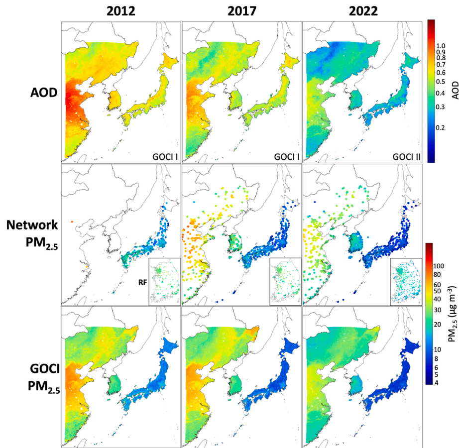
Fig. 6. GOCI gap-filled aerosol optical depth (AOD), PM_{2.5} from air quality networks, and GOCI PM_{2.5} obtained by applying a RF algorithm to the GOCI AOD data. Data are annual means for 2012 (the first year with complete GOCI data), 2017, and 2022. The gap-filled AOD data provide continuous 2 \times 2 \text{ km}^2 coverage of eastern China, S. Korea, and Japan for 2011–2022. The PM_{2.5} network data are from individual sites and enlarged for visibility. The S. Korea insets in the middle panels provide greater resolution of network data gaps. PM_{2.5} measurements from the AirKorea network started in 2015, and the S. Korea PM_{2.5} network data shown for 2012 are from a RF reconstruction as described in Section 2.3.
