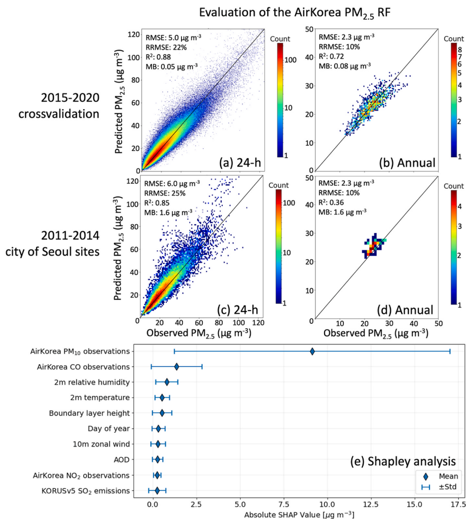
Fig. 2. Evaluation of the AirKorea \text{PM}_{2.5} RF predictions. The top panels evaluate the AirKorea \text{PM}_{2.5} RF predictions in the 2015–2020 training period at grid cells withheld entirely from training in a ten-fold crossvalidation procedure, aggregated at (a) 24-h and (b) annual resolution. Middle panels show an independent evaluation with observed 2011–2014 \text{PM}_{2.5} from the Seoul Research Institute surface network in the city of Seoul, selecting the 20 sites that are collocated with AirKorea sites on the 2 \times 2 \text{ km}^2 GOCI grid. Panels (a–d) show two-dimensional histograms where pixel color corresponds to the count of observation/prediction correspondences within the corresponding bin, with statistics inset and the identity line shown in black. The bottom panel shows the top ten predictors of AirKorea \text{PM}_{2.5} ranked by importance by the SHAP analysis. Predictor variable contributions are shown by mean absolute SHAP values and standard deviations. (For interpretation of the references to color in this figure legend, the reader is referred to the Web version of this article.)
