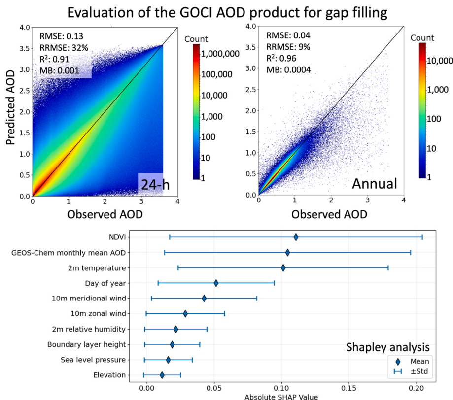
Fig. 1. Evaluation of the GOCI AOD RF predictions. The top panels evaluate the GOCI AOD RF predictions in the 2011–22 training period at grid cells withheld entirely from training in a ten-fold crossvalidation procedure, aggregated at (a) 24-h and (b) annual resolution. Results are shown as two-dimensional histograms where pixel color corresponds to the count of observation/prediction correspondences within the corresponding bin, with statistics inset and the identity line shown in black. The bottom panel shows the top ten predictors of AOD ranked by importance by the SHAP analysis. Predictor variable contributions are shown by mean absolute SHAP values and standard deviations. (For interpretation of the references to color in this figure legend, the reader is referred to the Web version of this article.)
