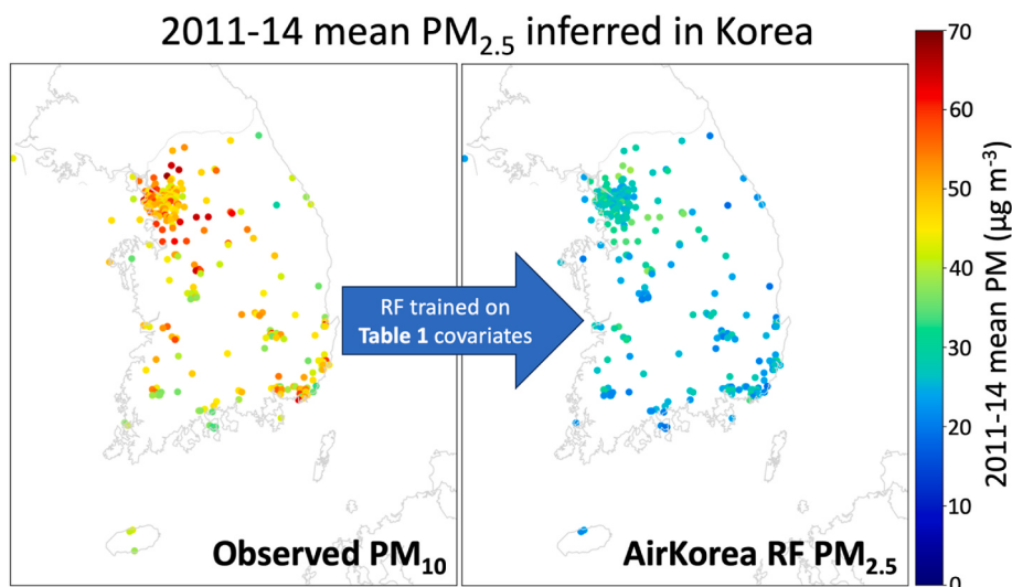
Fig. 3. 2011-14 mean observed \text{PM}_{10} and inferred \text{PM}_{2.5} at AirKorea sites. The AirKorea \text{PM}_{2.5} RF is trained on data in Table 1 and its Shapley analysis is in Fig. 2.
