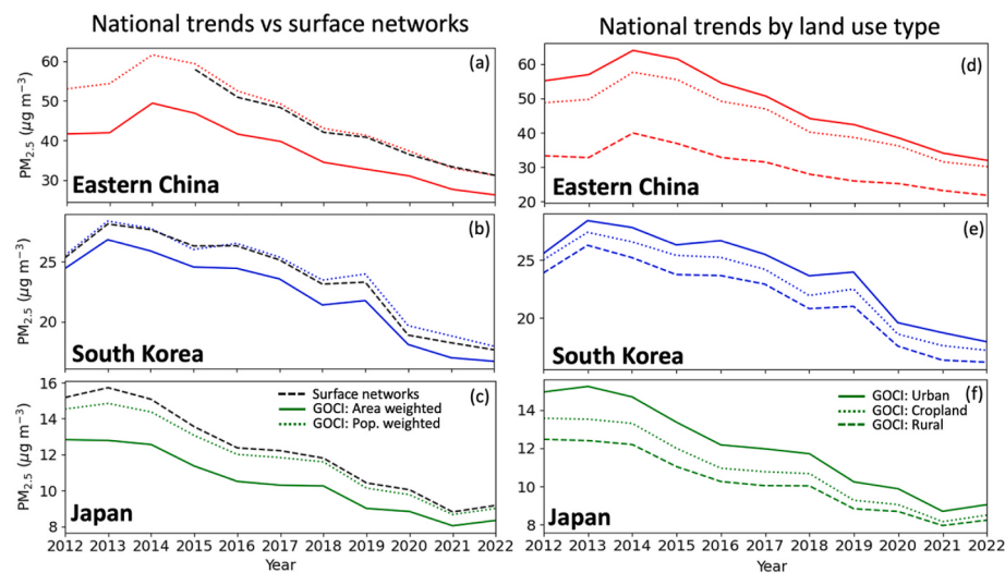
Fig. 7. Trends in annual mean GOCI PM_{2.5} concentrations averaged over eastern China, South Korea, and Japan for years with complete data (2012–2022). Also shown are the trends from the national PM_{2.5} networks (dashed black lines) averaged over 2 \times 2 \text{ km}^2 grid cells and requiring at least 80% of data for a given year. Surface network data in South Korea prior to 2015 are generated from the AirKorea PM_{2.5} RF using PM_{10} and other covariates (Table 1). GOCI PM_{2.5} are shown as averages weighted by area, population, and land type.
