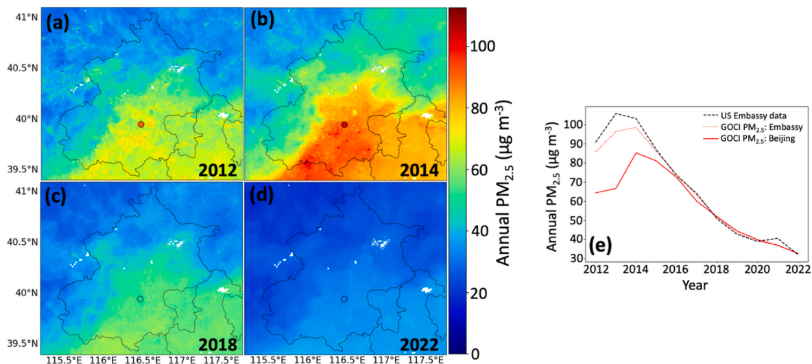
Fig. 8. Annual mean GOCI PM_{2.5} in Beijing compared with US embassy PM_{2.5} observations in individual years. The left panels show the distribution of PM_{2.5} in the city of Beijing (centered black outline) and surrounding area, with the location of the US embassy shown as a black circle. The right panel shows long-term trends at the US embassy site and averaged within Beijing city limits.
