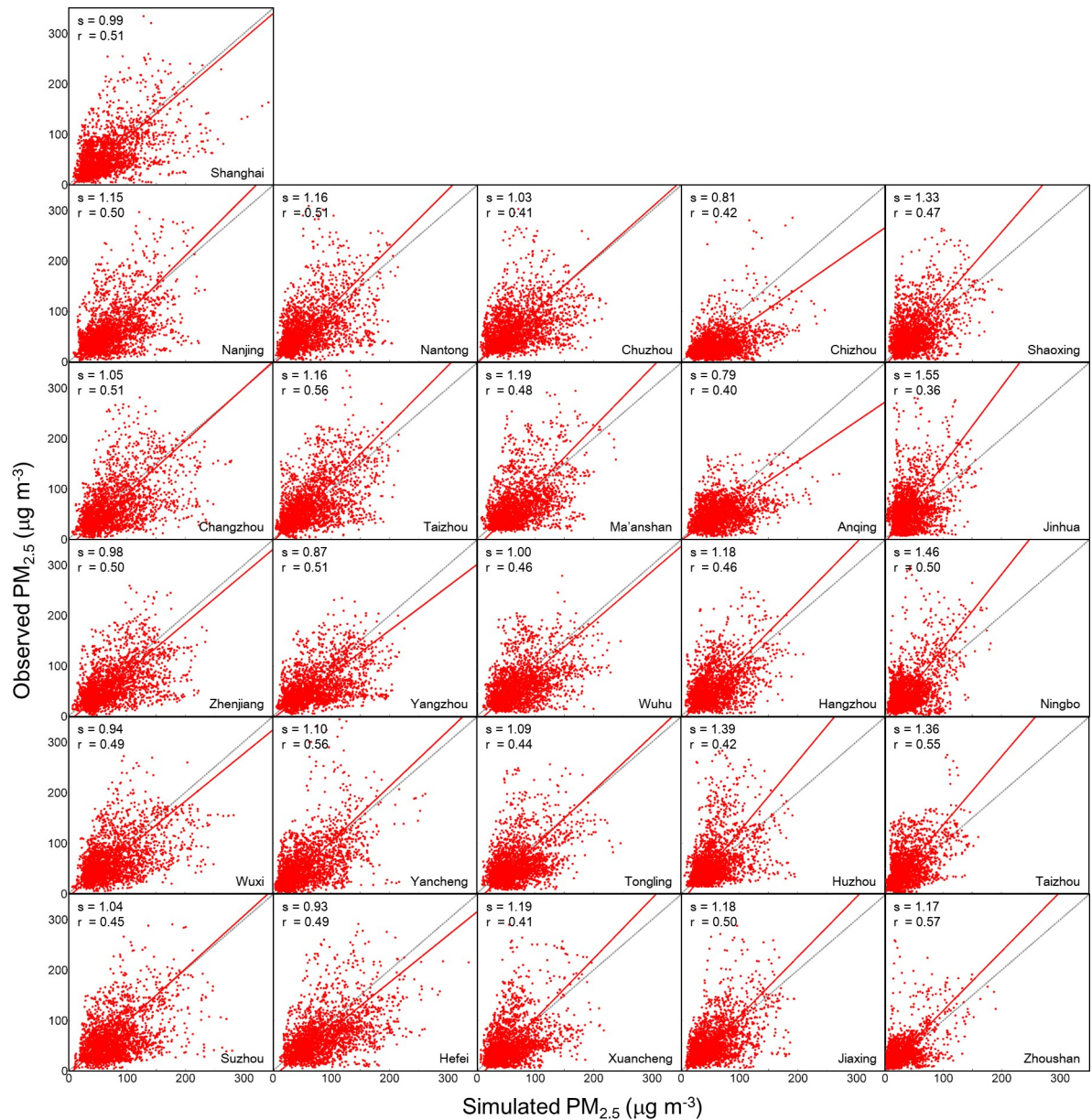
Fig 3. Scatter plots of simulated versus observed hourly PM 2.5 concentrations at the 26 cities in the YRD region. Also shown are the reduced-major axis regression lines (solid lines), the regression slopes (s) and correlation coefficients (r). Grey dashed lines indicate the 1:1 ratio.
