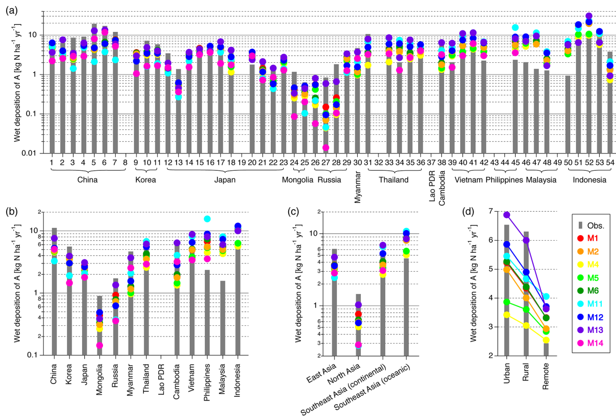
Figure 7. Model evaluation of the annual accumulated wet deposition of ammonium aerosol and ammonia ( \text{NH}_3 ) (A) (a) at each EANET observation site, (b) for countries, (c) over four defined regions, and (d) over different site classifications.
